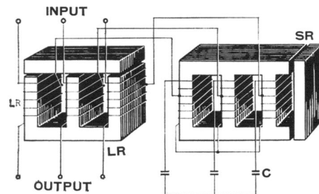
Circuit diagram of VN33
