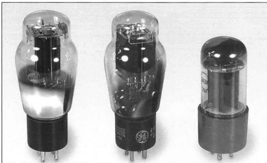
Tung-Sol Bi-Plate 2A3 (1940s); GE Box Bi-Plate 2A3 (1940s); Sylvania 5930/2A3W (1940s)
