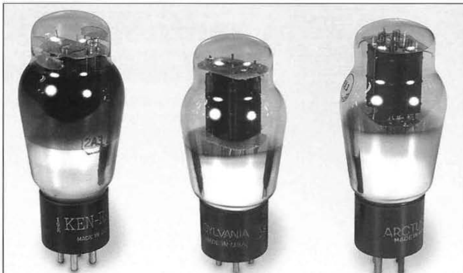
Ken-Rad Bi-Plate 2A3 (1940s); Sylvania Bi-Plate 2A3 (1940s); Arcturus Bi-Plate 2A3 (1938)
