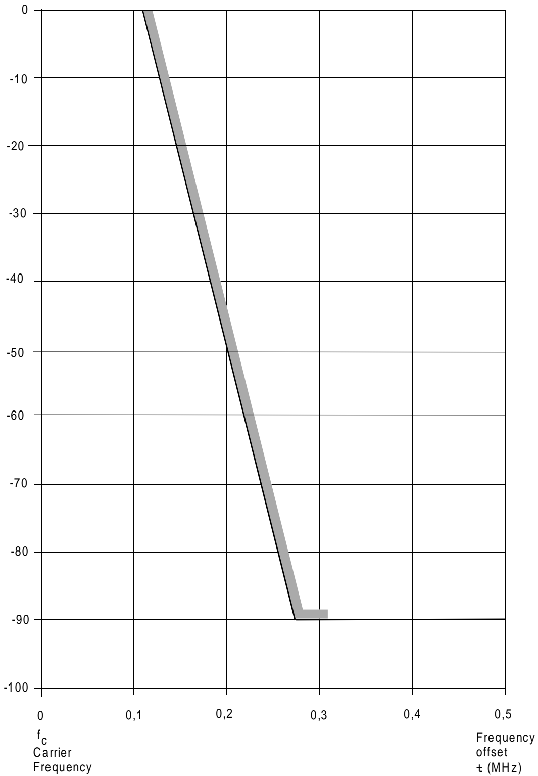
Figure 4: Limits on transmitter spectrum due to abnormal AF input levels (see subclause 4.9)
