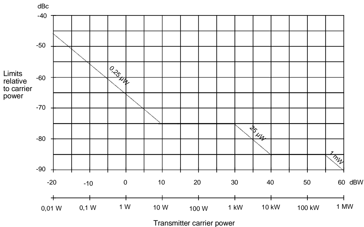
Figure 1: Limits for spurious emission within the frequency range 87,5 to 137 MHz
