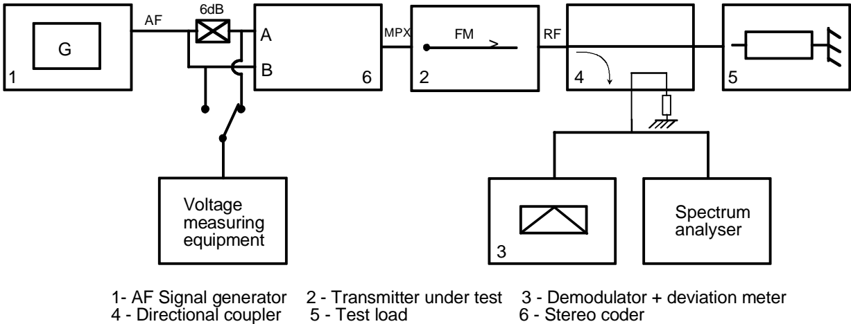
Figure 6: Measuring arrangements for stereophonic transmitters
